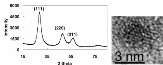
Figure 1. XRD pattern (left) and HRTEM image (right) of the as-synthesized ZnS nanoparticle.
